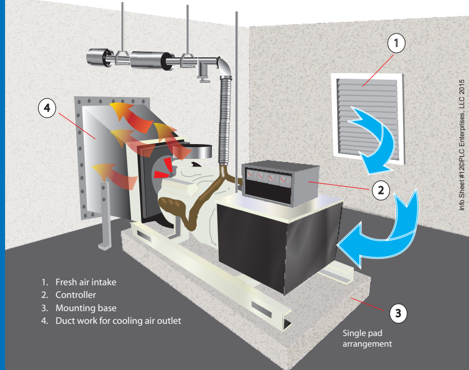
Diagram 3 Sample stationary generator set inside installation
