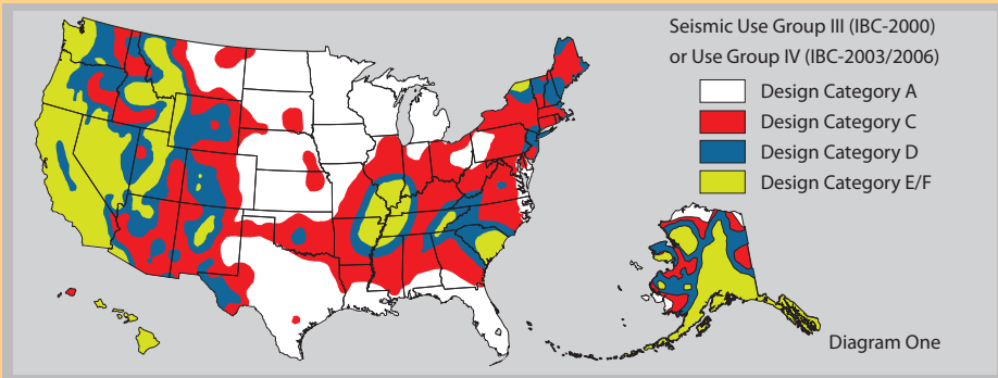
Diagram two - US Seismic areas
