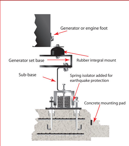
Diagram one - Seismic arrangement for vibration isolators
