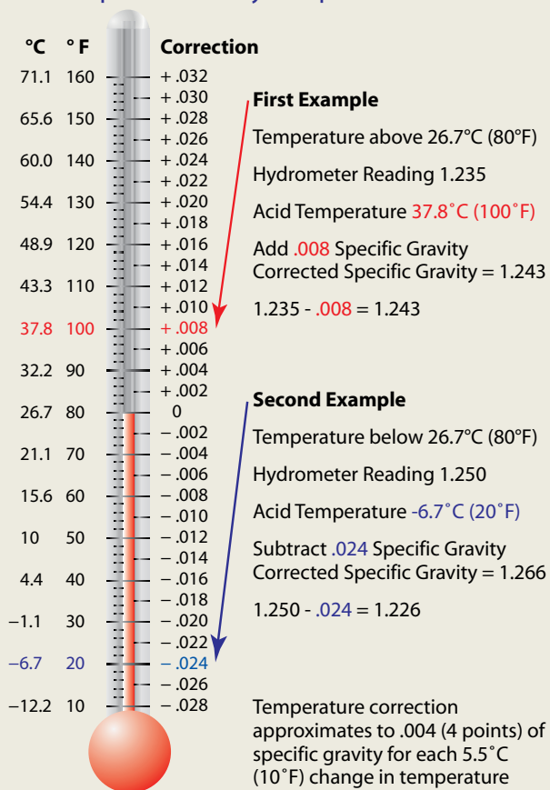
Chart 3- Specific Gravity Temperature Correction
