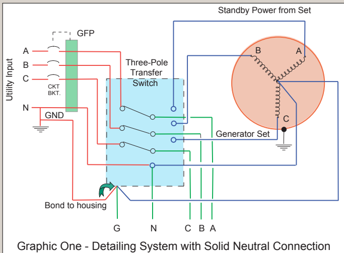
Graphic One - Detailing System with Solid Neutral Connection
