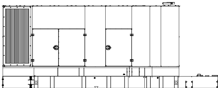
Enclosure with State Tank (12- 48 Hour)
