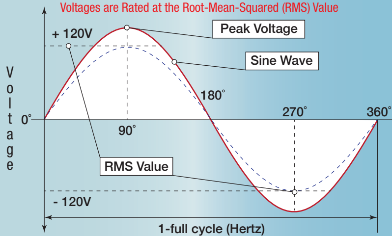
AC Voltage Sine Wave 120V Single Phase
